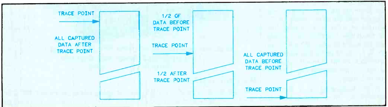
Figure 10. Because the logic analyzer stores data as it goes, it is possible to display data captured before the trigger point as well as data captured after the trigger point.
