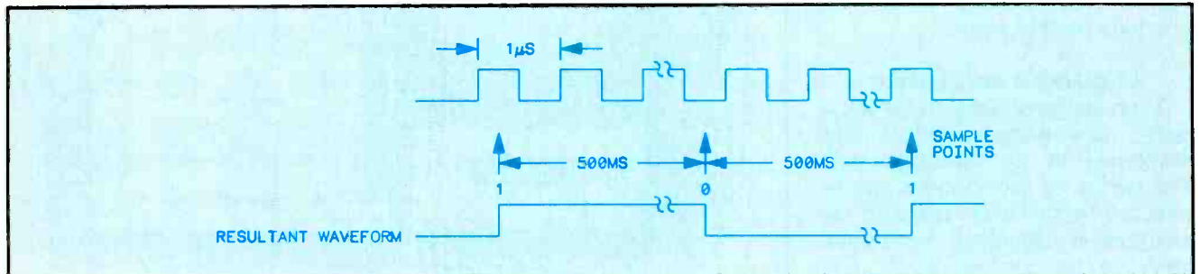
Figure 6. If the sample period is long compared to the period of the waveform being sampled, inaccuracy may result because the sampled lines may change many times in between sample points.
