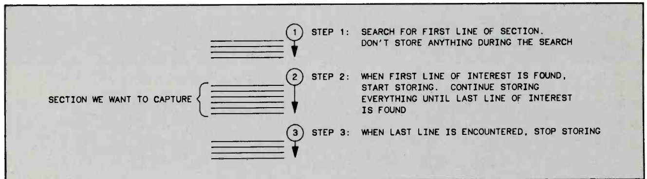
Figure 18. Analyzers are capable of selective storage, that is, storing only specific portions of an entire program (routines). This assists in troubleshooting areas where problems occur.
