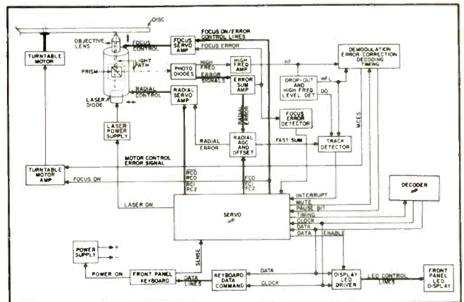
Figure 1. The NAP compact digital audio disc player shown in this block diagram features two microcomputers: one to control the motion of the laser stylus and one to handle the audio mute and pre-emphasis information.
